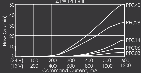
Typical Metering Performance (①→②)
