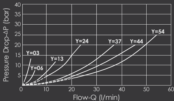
Port ③ Inlet Performance Chart
